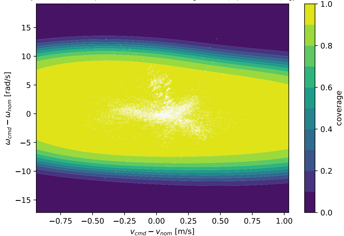
Residual coverage vs command offset (0 = off / OOD; state fixed at mean [0.56 m/s, 0.46 rad/s])
